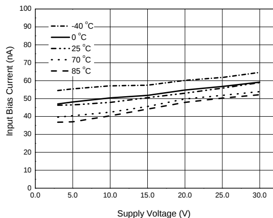
Supply Voltage vs. Input Bias Current
