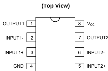
PDIP-8
